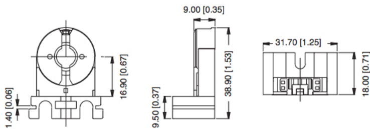
FL206X* Δ Flush Sides, Slot Mount 18 ga. Panel
