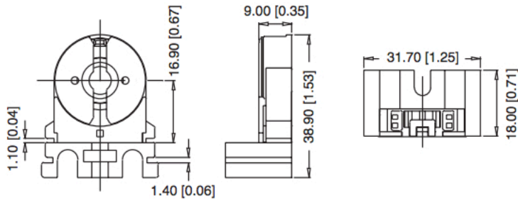
FL206* Δ Solid Shoulder, Slot on Mount 18 or 20 ga. Panel, Nut Slot
