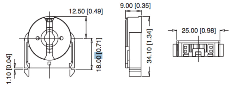
FL206-BSI* Snap-in Mount from the Top
